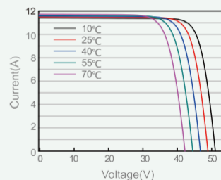
Current-Voltage Curve(SP455M-72H)
