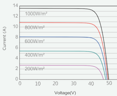
Current-Voltage Curve(SP540M-72H)
